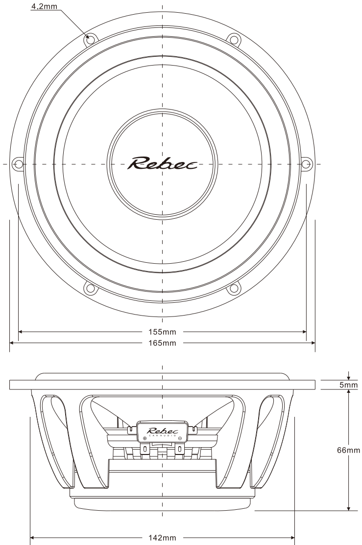
Speaker Dimension Drawing
